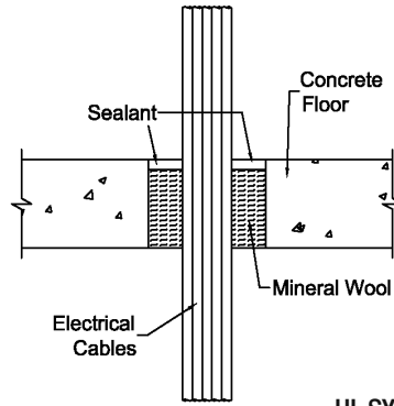
Fig. 2: MISCELLANEOUS METALLIC PIPE & CABLE PENETRATIONS
